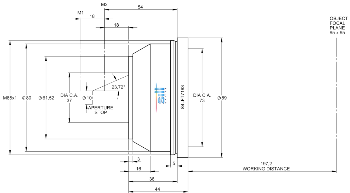
outline drawing
